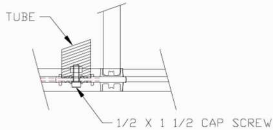
DETAIL A: ATTACHING END CASTINGS AND FASTENING TUBES
