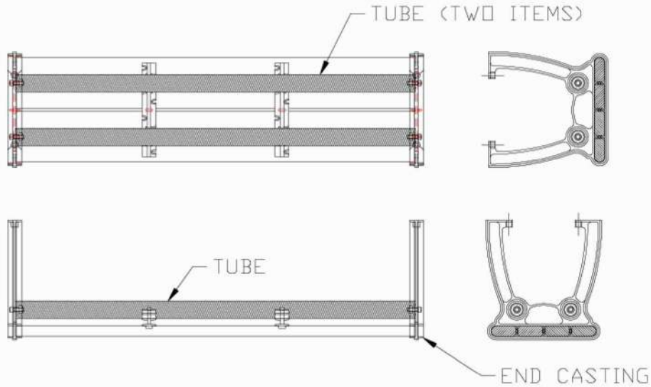
DETAIL A: ATTACHING END CASTINGS AND FASTENING TUBES
