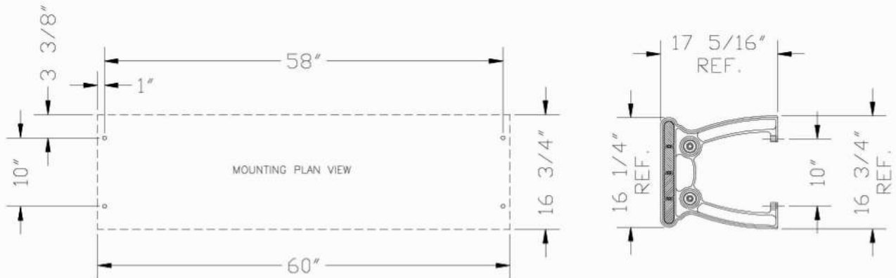
DIAGRAM 3: SEAT 5 FOOT LENGTH 300001, SURFACE MOUNTING
