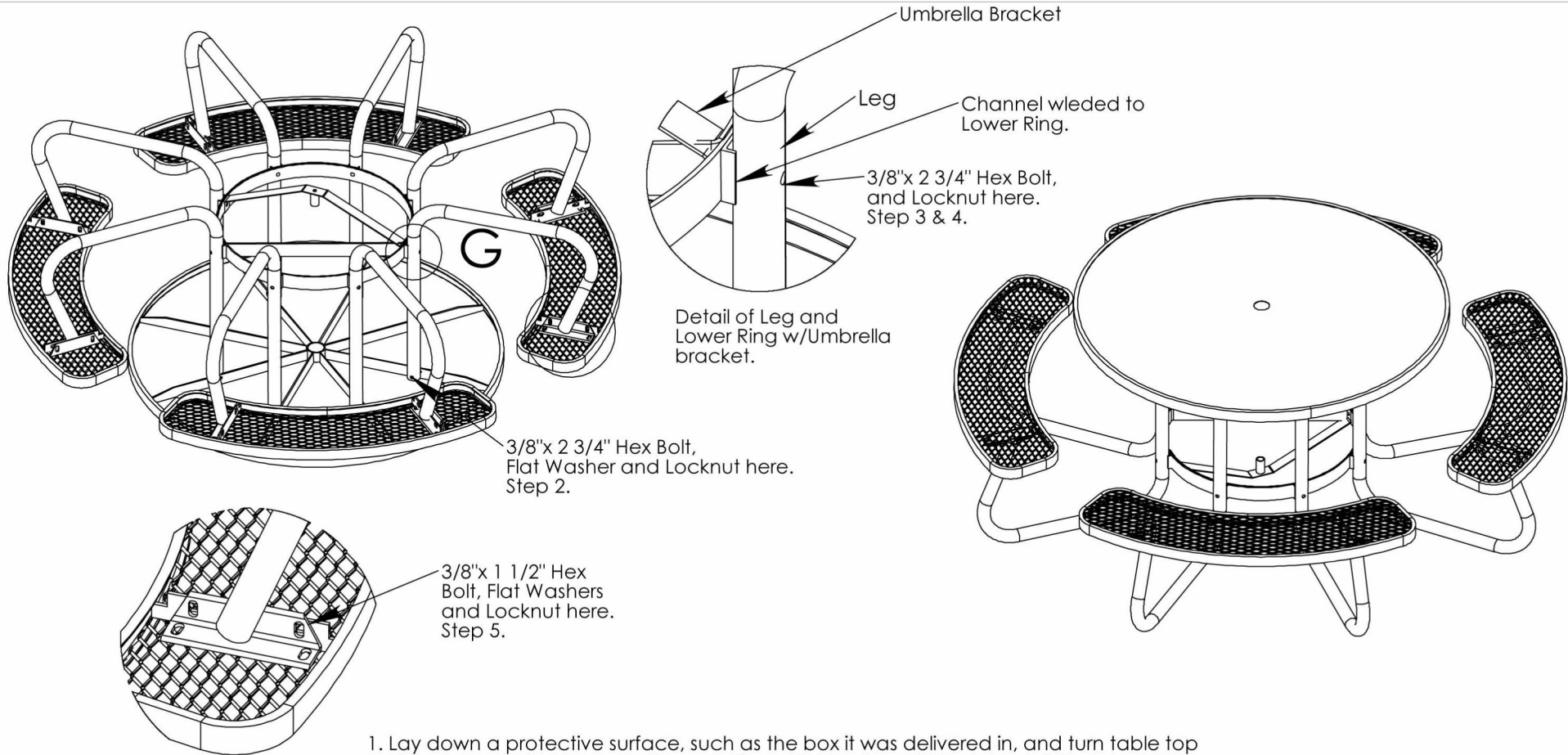
Detail of Seat Mounting Bracket
