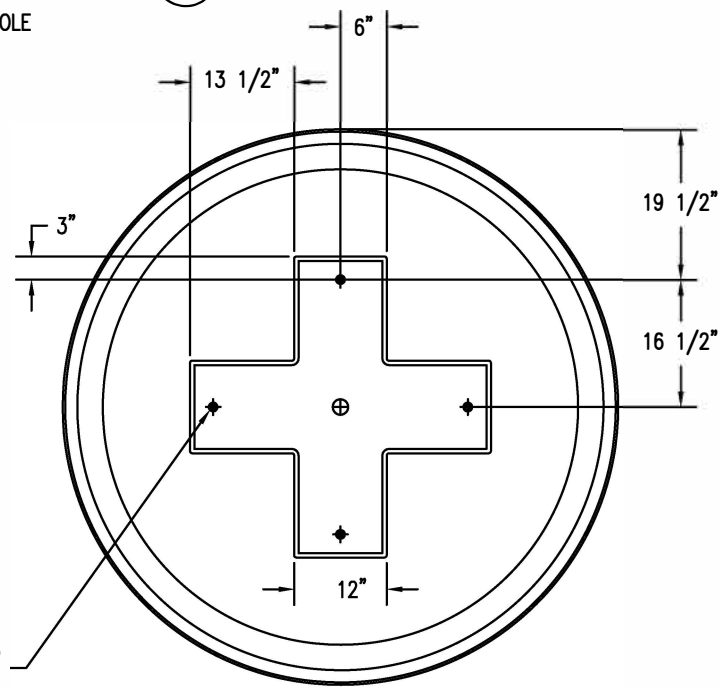
3 BOTTOM VIEW
