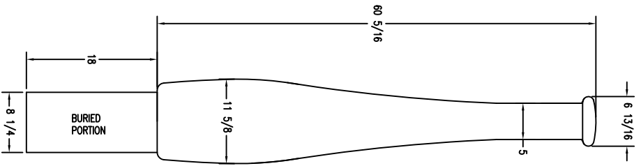
1 ELEVATION VIEW OF BOLLARD SCALE: NTS
