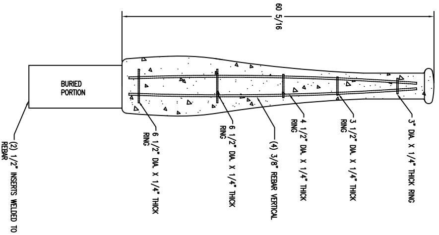
3 SECTION VIEW OF BOLLARD SCALE: NTS
