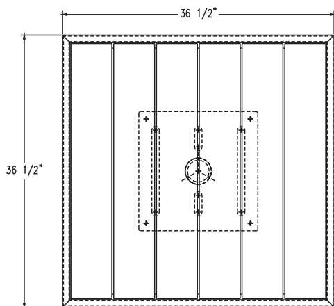
TOP VIEW 1041
