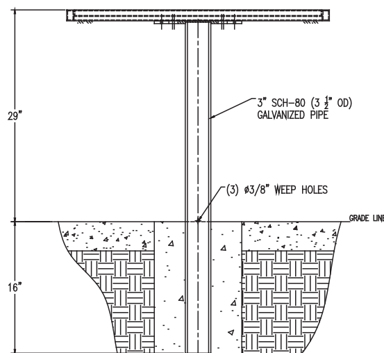
ELEVATION VIEW
