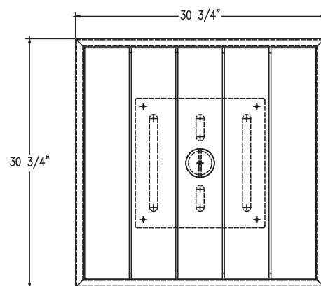
TOP VIEW 1045
