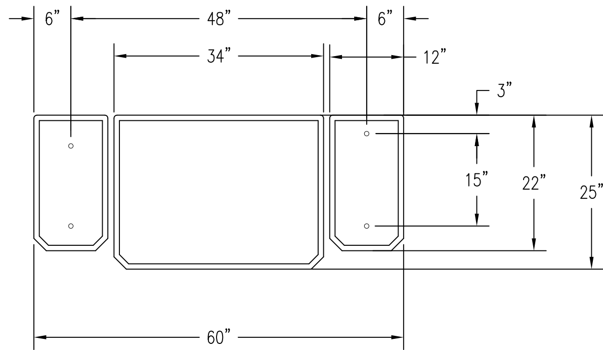
1 TOP VIEW OF TABLE Scale: 1/16" = 1"
