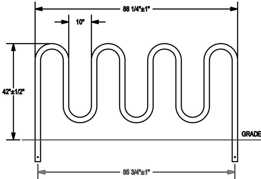
ELEVATION VIEW
