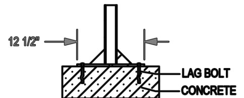
□ SURFACE GUSSET MOUNT (SG)
