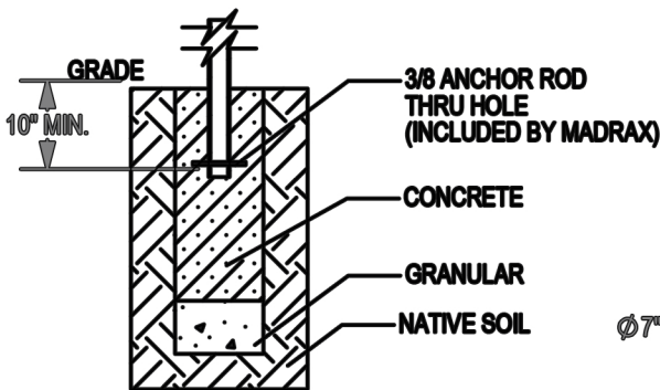
□ IN GROUND MOUNT (IG)
