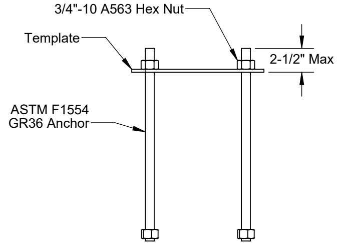
Anchor Bolt Template Assembly
