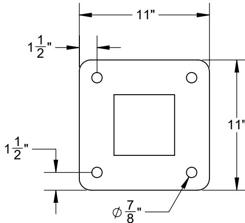
3/4" Base Plate
