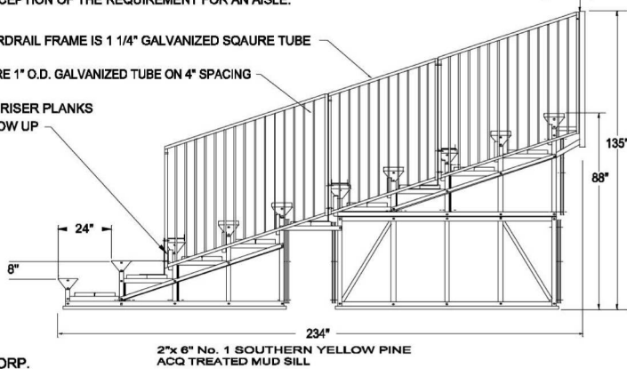
BLA10 with V4 and F4 options 10 ROW BLEACHER FRAME
