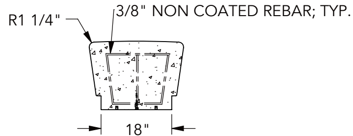
⑤ SECTION
