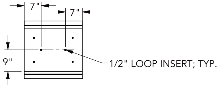
③ BOTTOM VIEW
